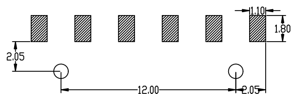
6PIN P.C.B. LAYOUT (TOP VIEW)
